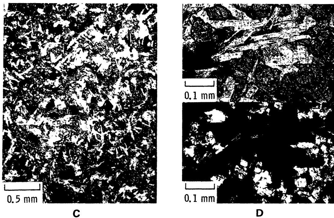
Fig. 3. Lonar basalt, laboratory shocked. Upper plates, Class 1. Lower plates, Class 2. (A) Texture of sample shocked to 202 kbar, Class 1, basically unchanged from initial texture (Fig. 1). Plane polarized light. (B) Sample did not include a large phenocryst, as shown in the naturally shocked Class 1 sample, Fig. 2, but some fracturing is visible in the fine-grained groundmass shown here. Top, plane polarized light. Bottom, polarizers crossed at 80°. Note slight undulatory extinction in plagioclase in groundmass. (C) Texture of sample shocked to 270 kbar, Class 2, showing similarity to initial texture (Fig. 1). (D) Plagioclase laths are undeformed, but are converted to maskelynite. Top, plane polarized light. Bottom, polarizers crossed at 80°.
