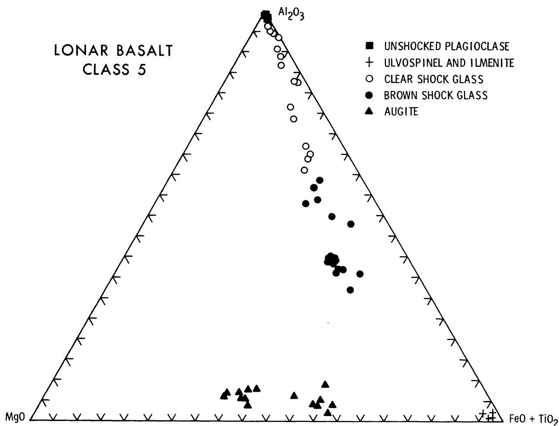
Fig. 9. Ternary diagram showing composition variation of colorless and brown shock glasses with respect to the major minerals in Class 5 samples of naturally shocked Lönar basalt.
