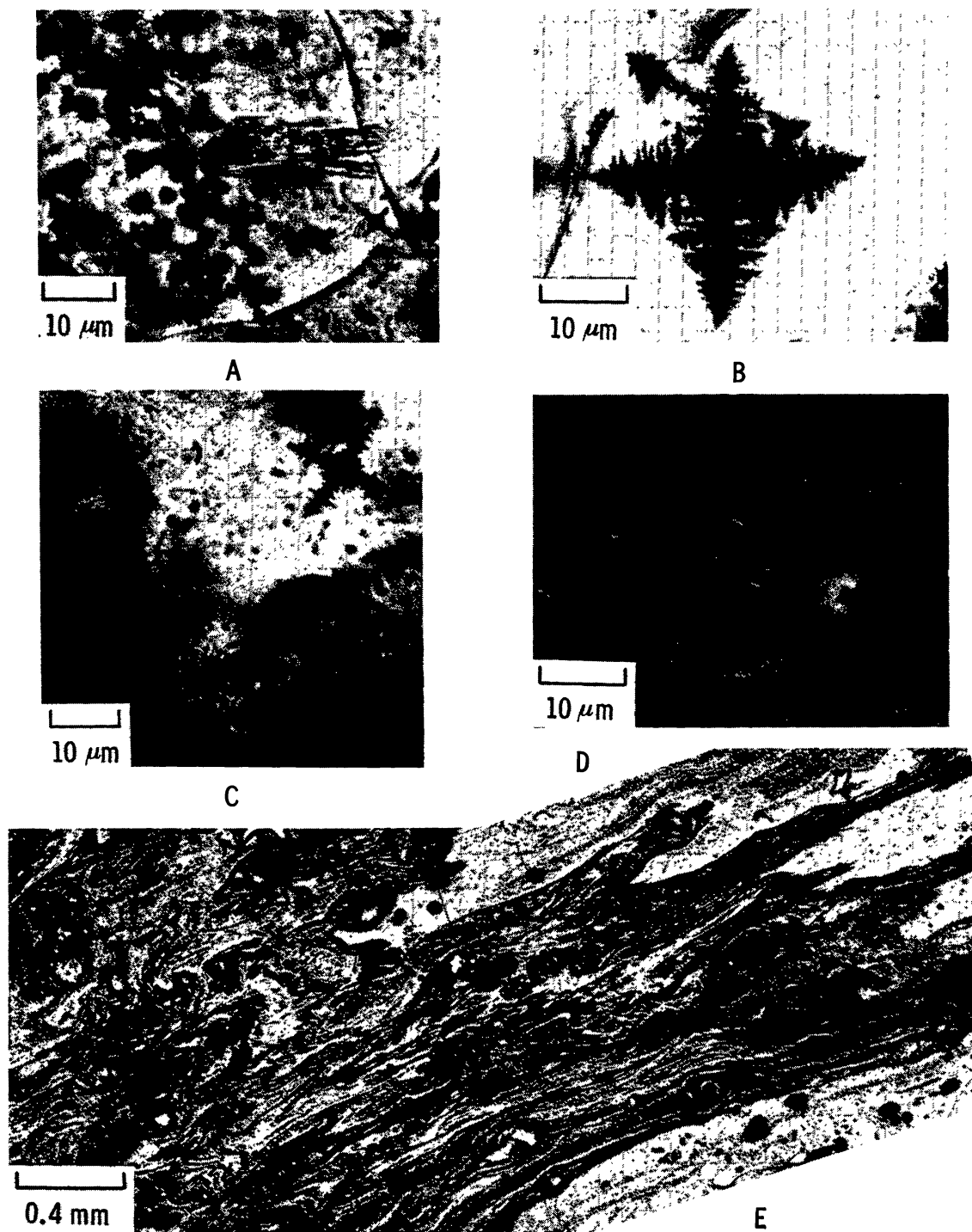
Fig. 8. LONAR basalt, naturally shocked, Class 5. Dendrites and spherulites in shock-melted glass. (A) Dendritic titaniferous magnetite crystals and a bow-tie spherulite within brown glass. Plane polarized light; oil immersion. (B) The largest dendritic titaniferous magnetite crystal found in the shock-melted glass. Plane polarized light; oil immersion. (C) An opaque dendrite, fan spherulites with scalloped edges (lower right and left margin), and a plumose spherulite with feathery edges (bottom center). Plane polarized light; oil immersion. (D) Titaniferous magnetite crystals aligned in flow bands in brown glass. Enlargement of region in (E). Plane polarized light; oil immersion. (E) Flow banding in shock-melted glass. This degree of heterogeneity is characteristic of the shock-melted glasses from LONAR. Plane polarized light.
