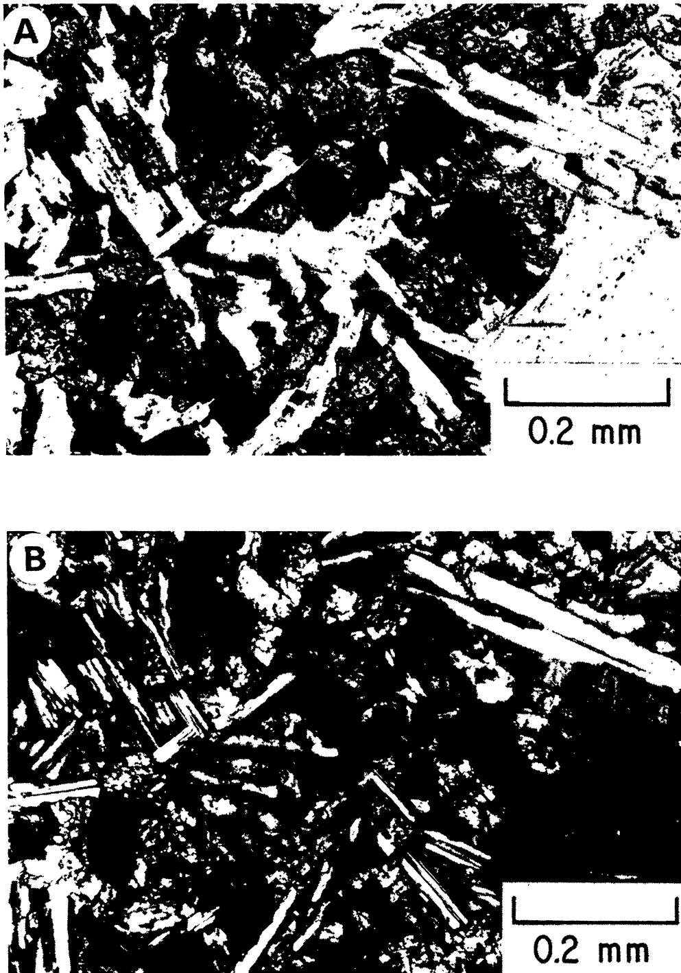
Fig. 1. Lunar basalt, unshocked, from a flow at 81 m depth. (a) Plane polarized light. (b) With polarizers crossed at 80°. Note microporphyrific texture, plagioclase laths and phenocryst, birefringent pyroxene grains, and opaque minerals.
